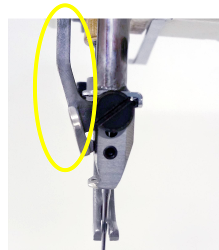
Needle thread catching system Prevents skip stitches by securing the needle thread feeding
